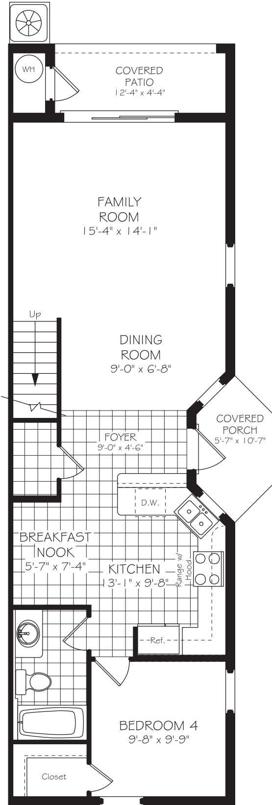
FIRST FLOOR
