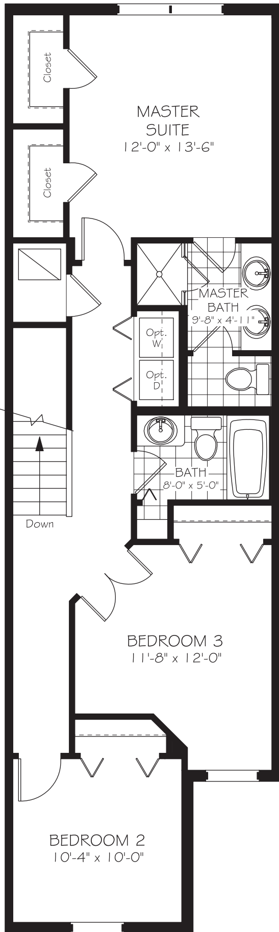
SECOND FLOOR
