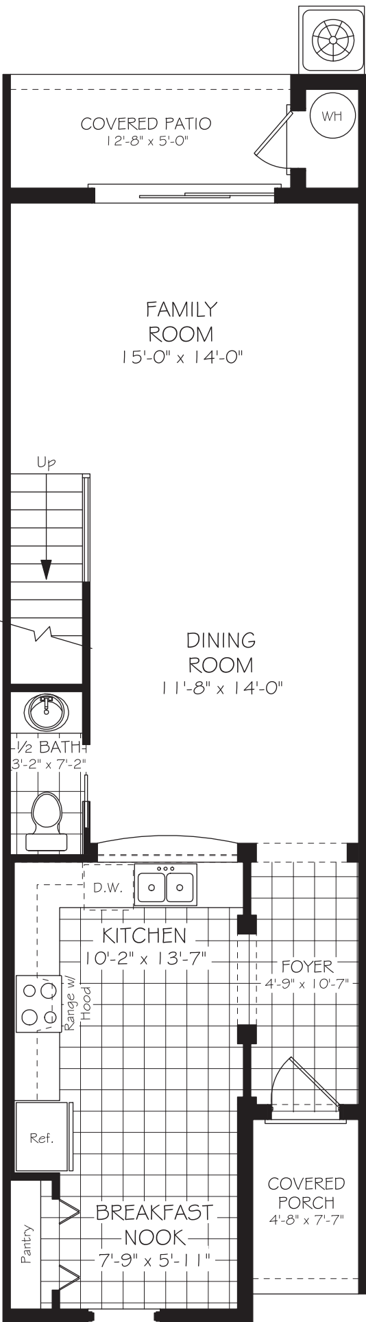
FIRST FLOOR
