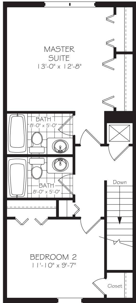
SECOND FLOOR
