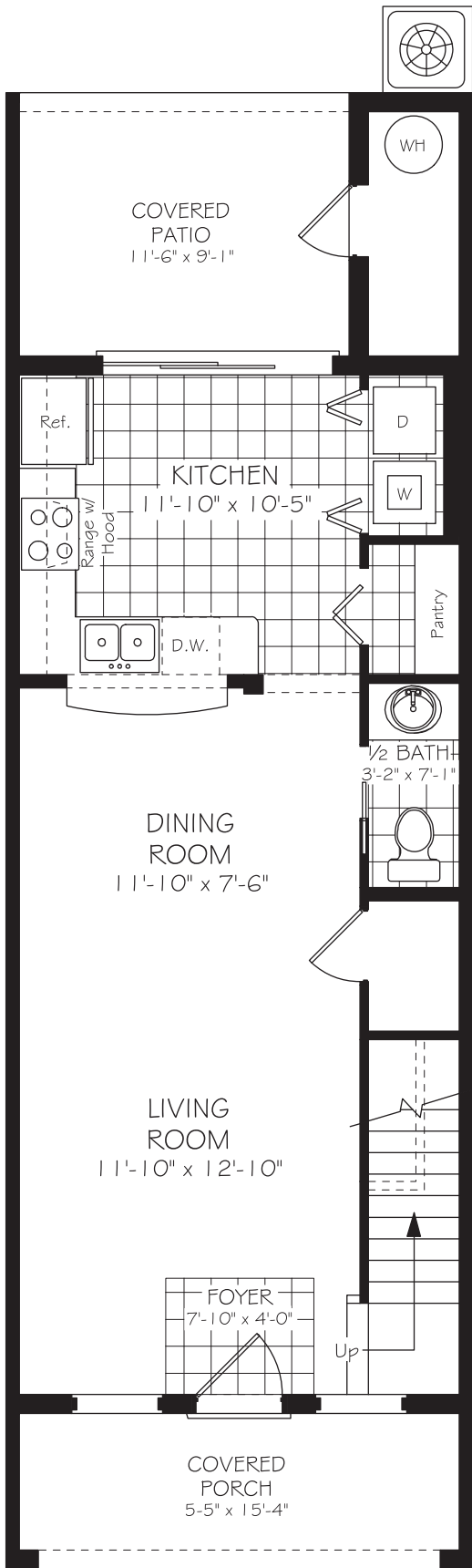
FIRST FLOOR
